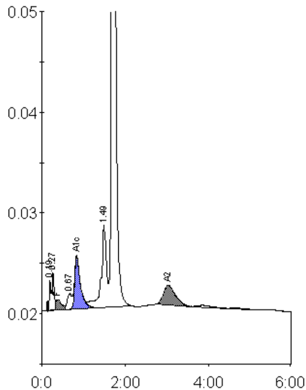
Peak table - ID: 10018725
