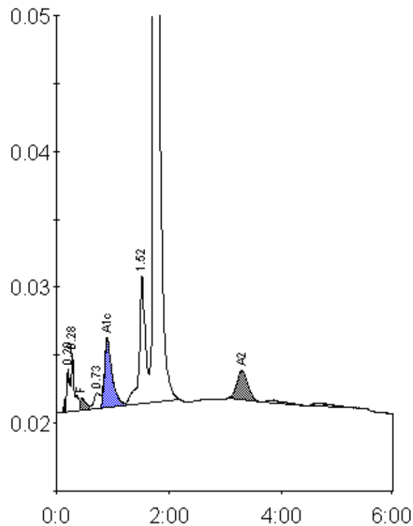
Peak table - ID: 10059979
