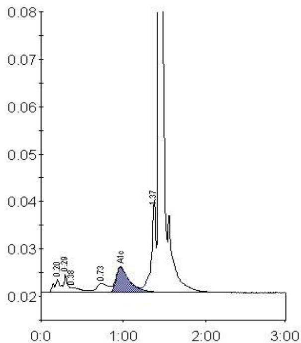
Peak table - ID: 10004574
