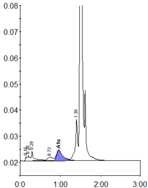
Peak table - ID: 10008639
