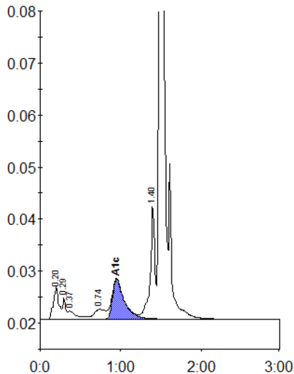
Peak table - ID: 10010088
