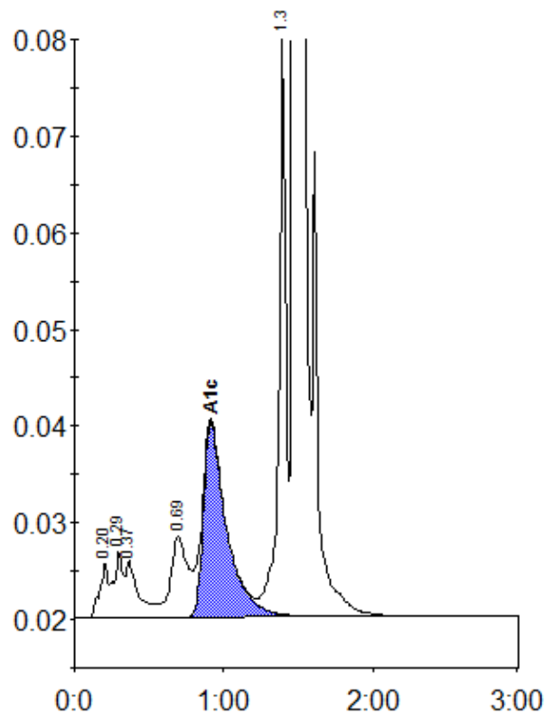
Peak table - ID: 10010724
