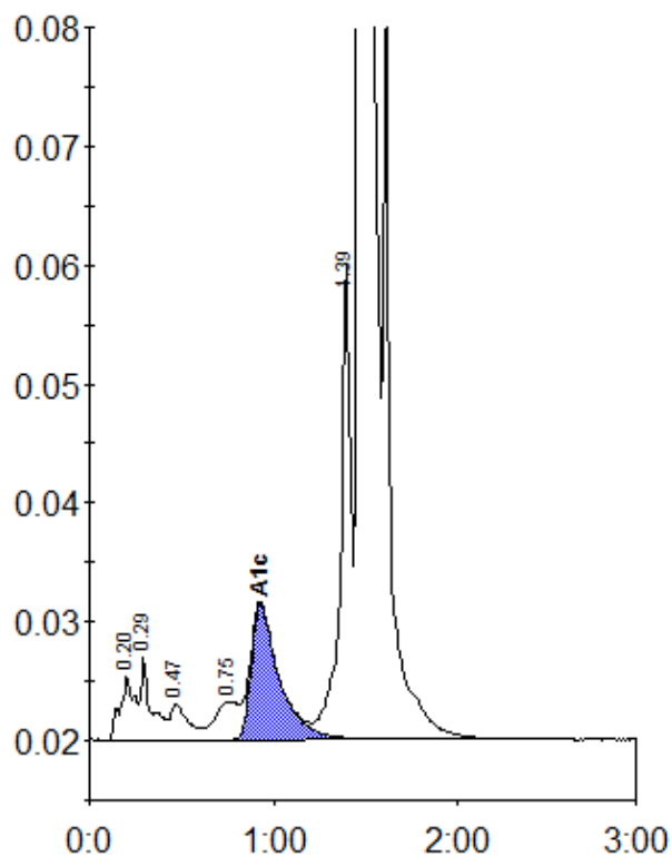
Peak table - ID: 10010944
