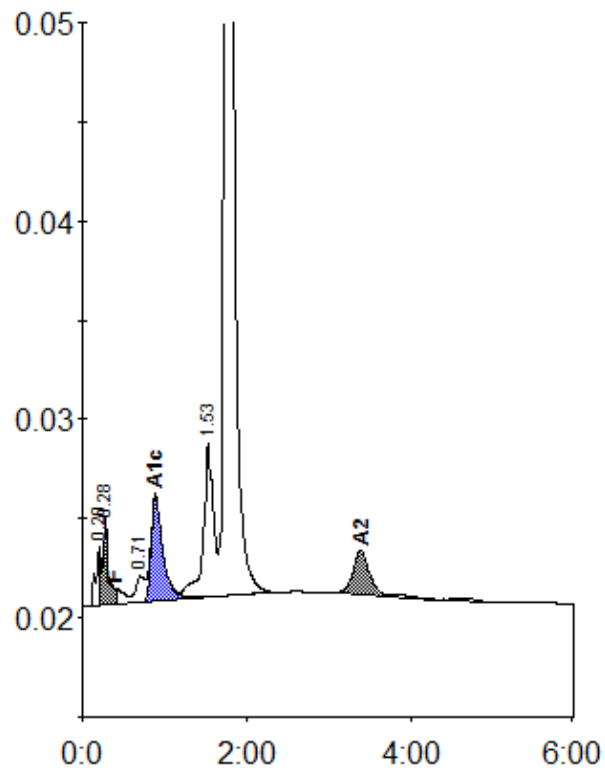
Peak table - ID: 10011860
