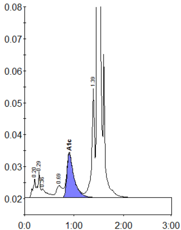
Peak table - ID: 10013904
