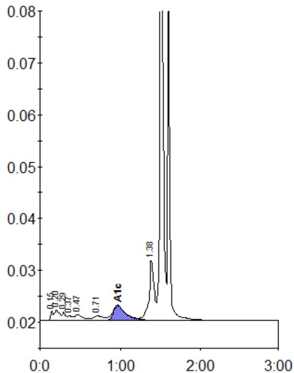
Peak table - ID: 10015269
