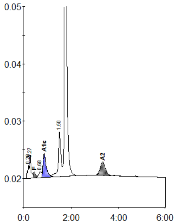
Peak table - ID: 10019645
