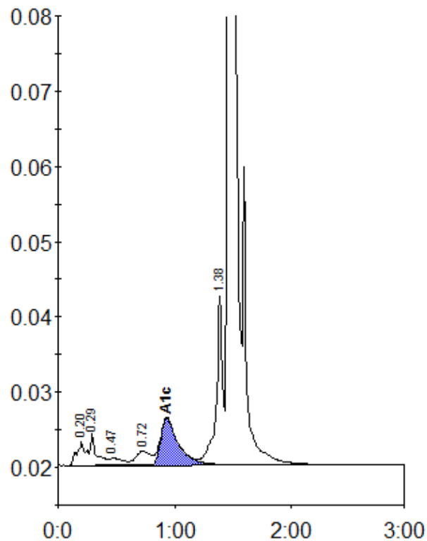
Peak table - ID: 10020471
