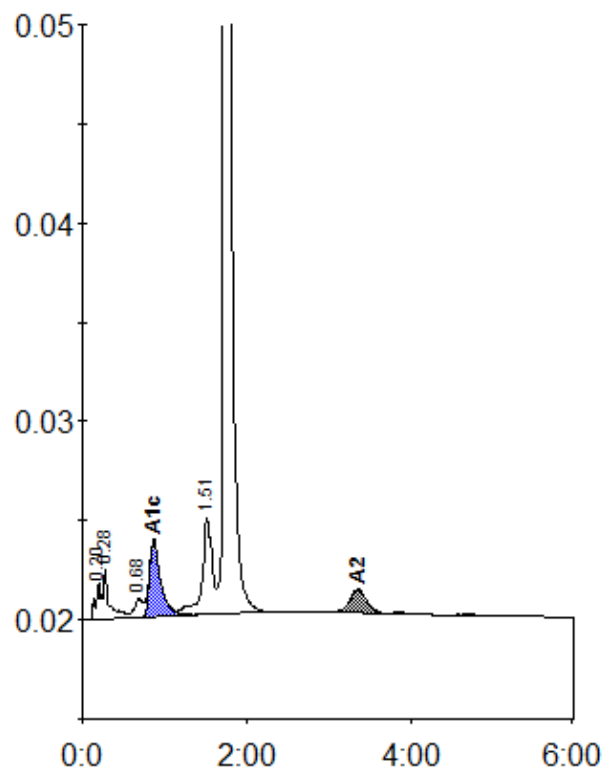
Peak table - ID: 10021528
