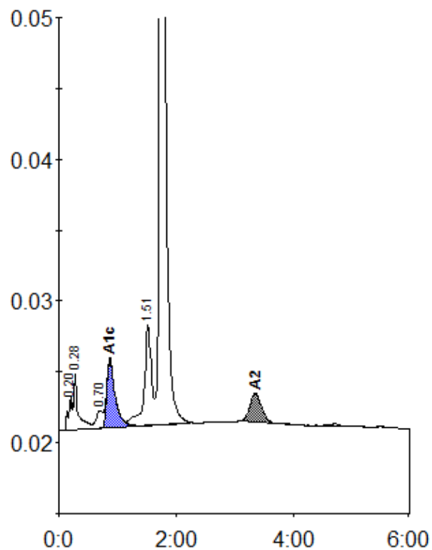
Peak table - ID: 10022179
