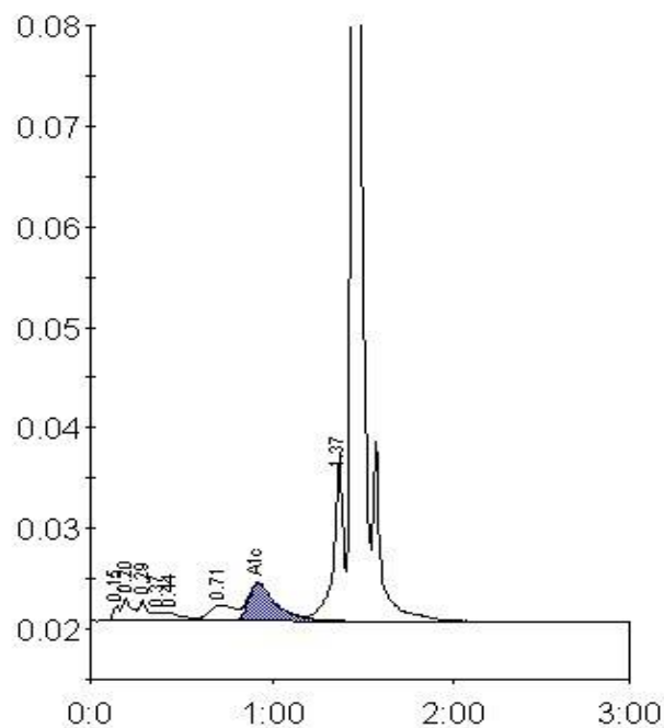
Peak table - ID: 10023482
