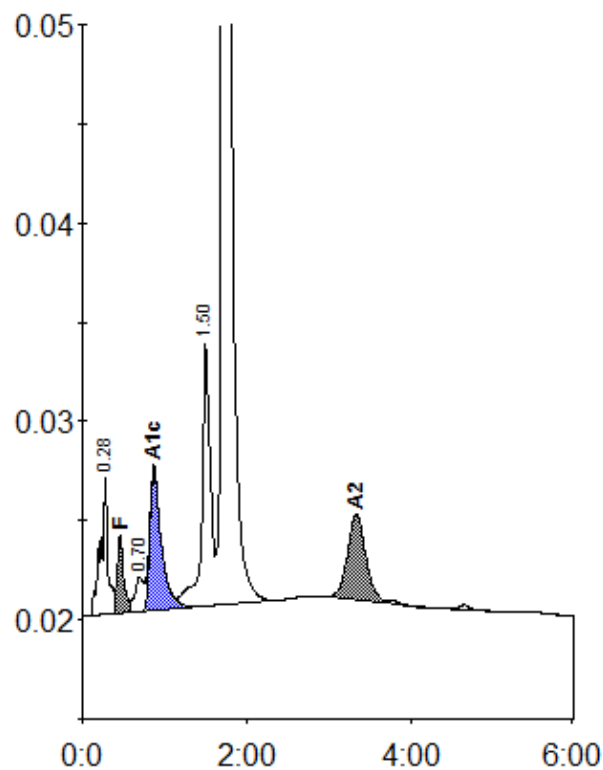
Peak table - ID: 10025423
