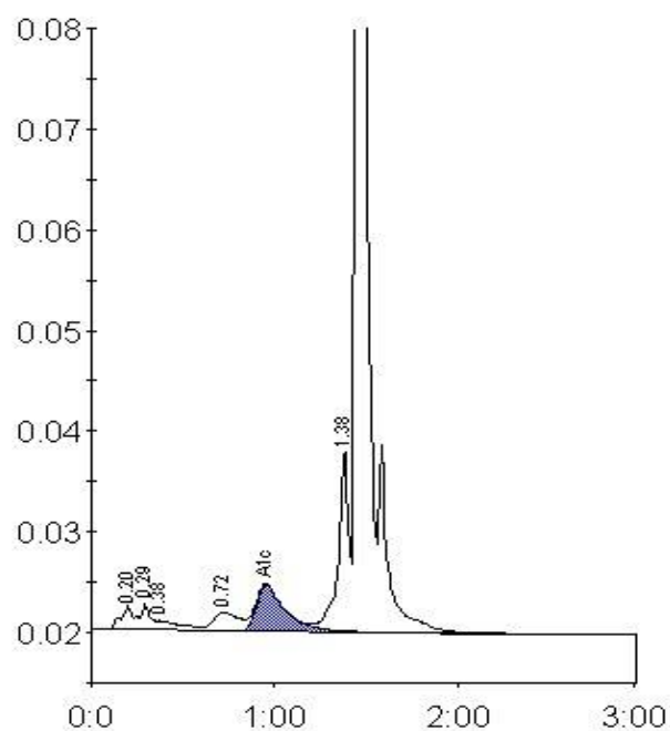
Peak table - ID: 10028654
