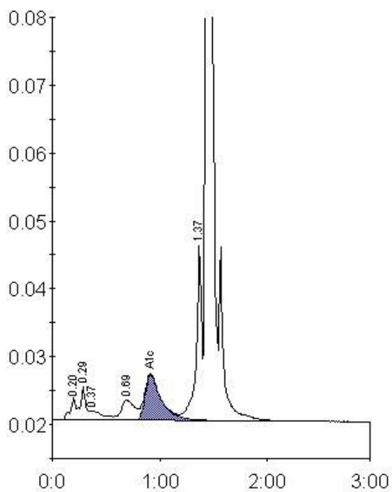
Peak table - ID: 10030430
