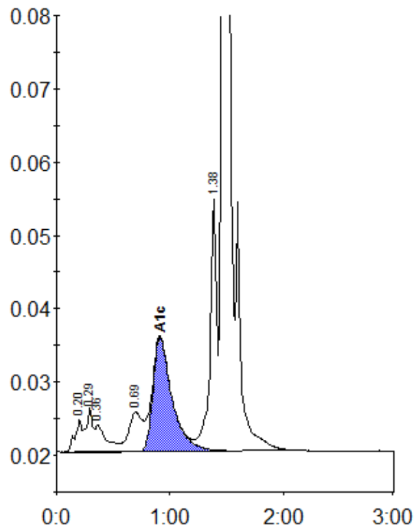
Peak table - ID: 10031304
