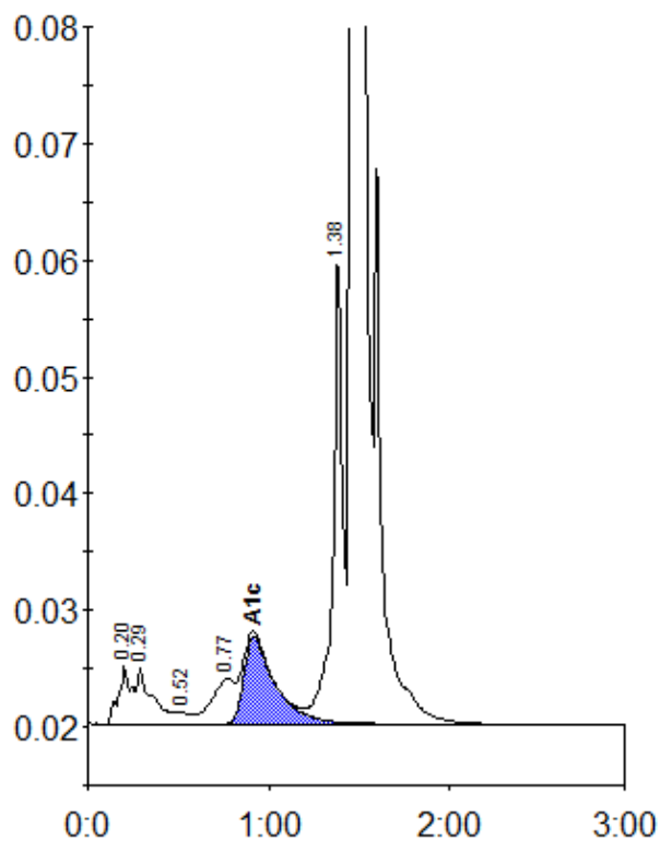
Peak table - ID: 10039453
