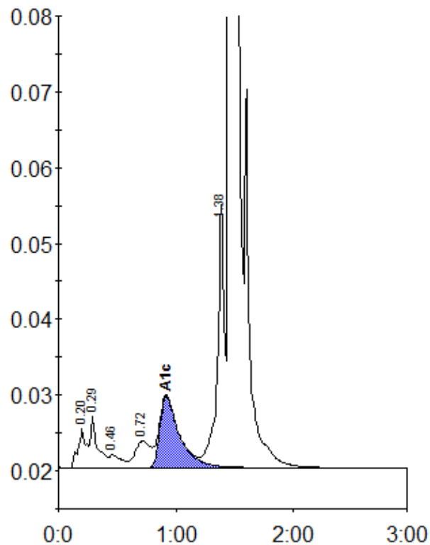
Peak table - ID: 10041119
