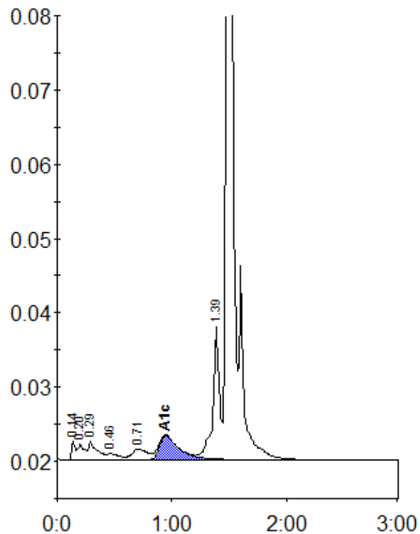
Peak table - ID: 10047742
