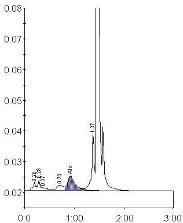
Peak table - ID: 10052509
