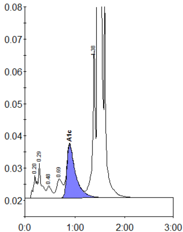
Peak table - ID: 10057471
