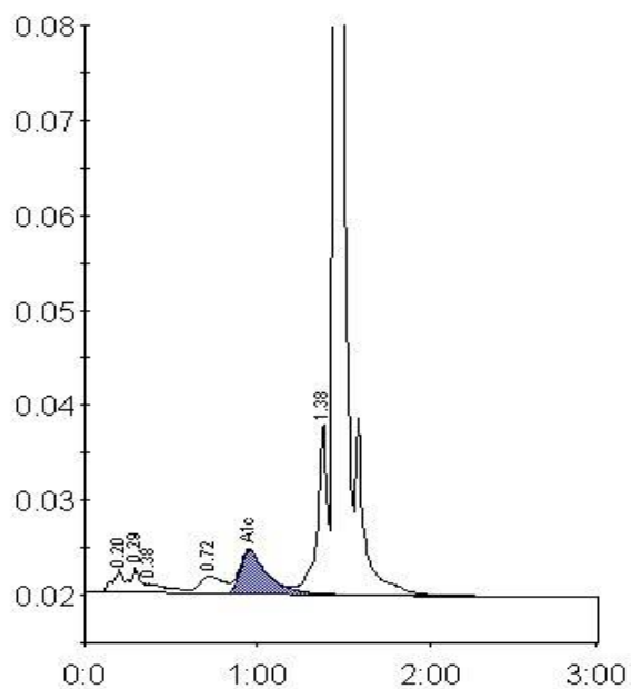
Peak table - ID: 10058028
