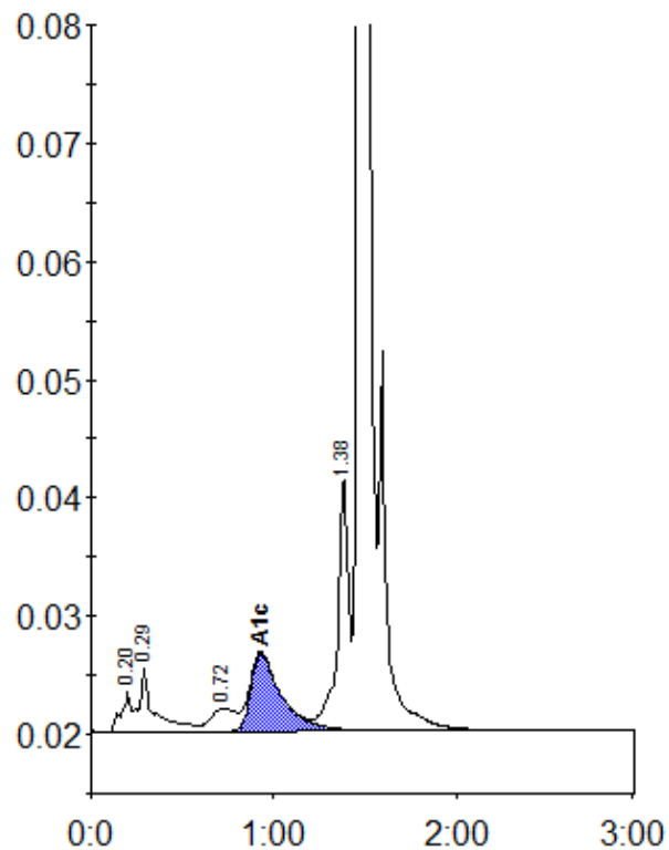
Peak table - ID: 10059907
