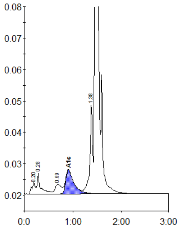
Peak table - ID: 10062274
