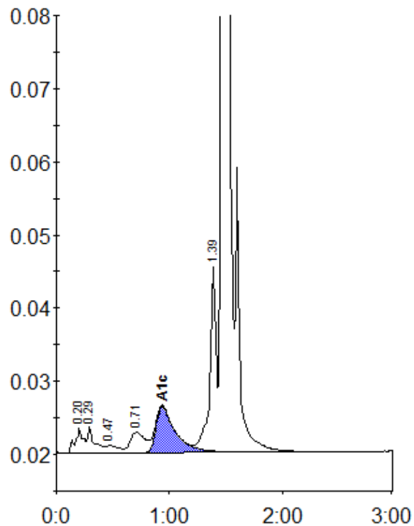
Peak table - ID: 10067109
