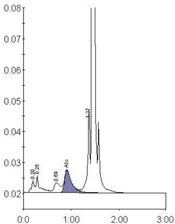
Peak table - ID: 10067517
