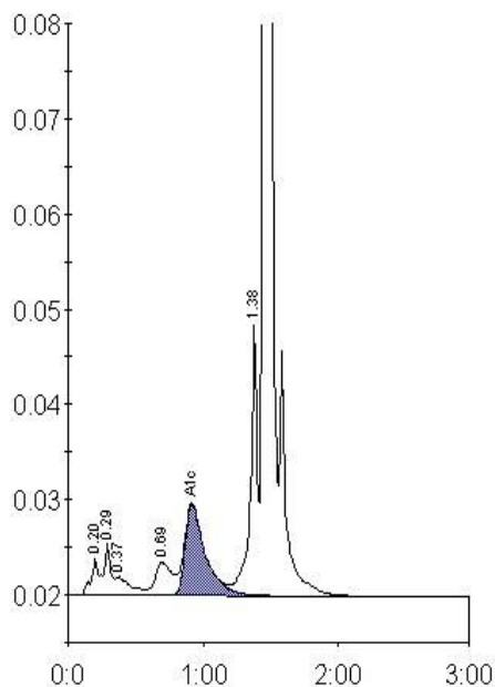
Peak R.time Height Area Area % A1a 0.20 3733 16721 1.1 A1b 0.29 5558 16101 1.0 Unknown 0.37 1925 15292 1.0 LA1c/CHb-1 0.69 3478 29309 1.9 A1c 0.92 9593 99319 8.8 P3 1.38 28461 104752 6.8 A0 1.45 413572 125665 581.7 Total Area: 1538150
