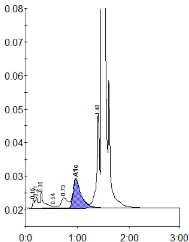
Peak table - ID: 10084099
