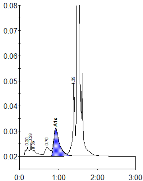
Peak table - ID: 10085504
