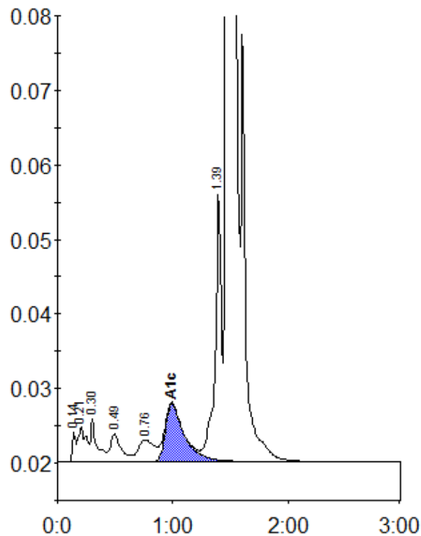
Peak table - ID: 10088638
