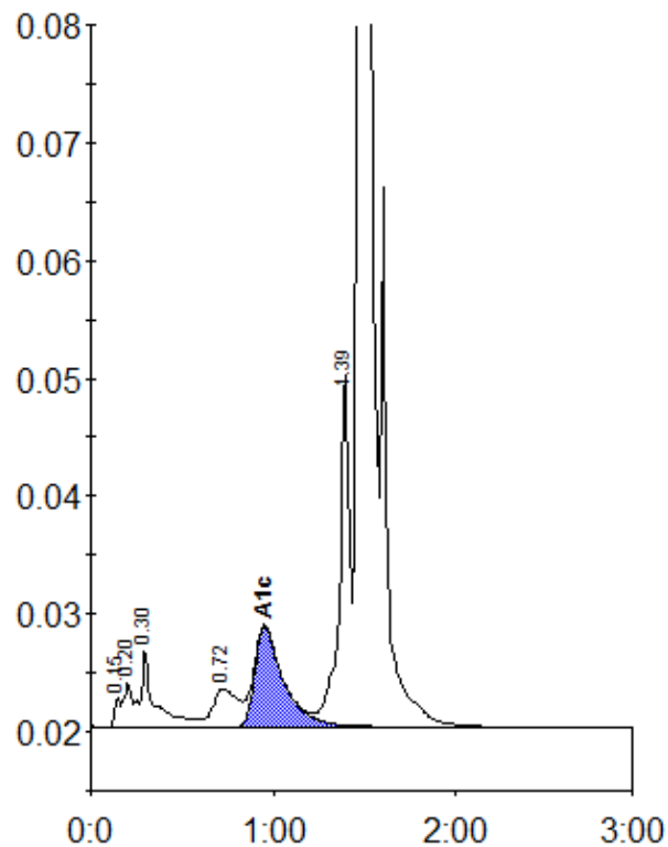
Peak table - ID: 10092549
