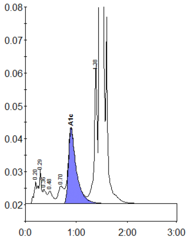
Peak table - ID: 10092696
