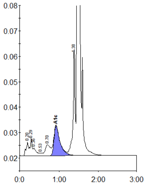
Peak table - ID: 10094295
