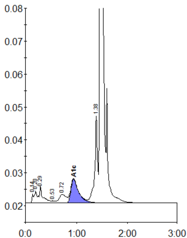
Peak table - ID: 10094986
