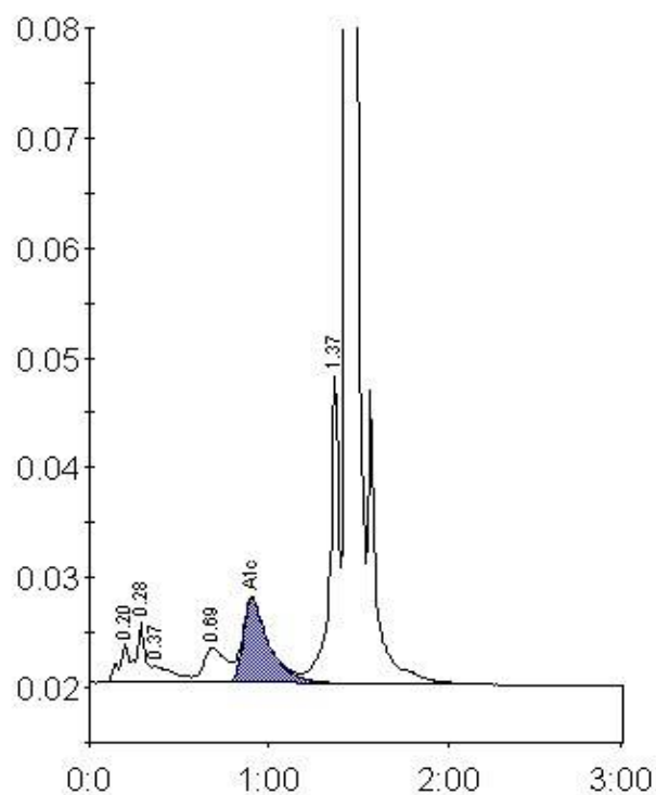
Peak table - ID: 10096170
