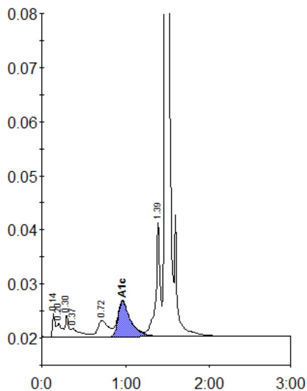
Peak table - ID: 10096912
