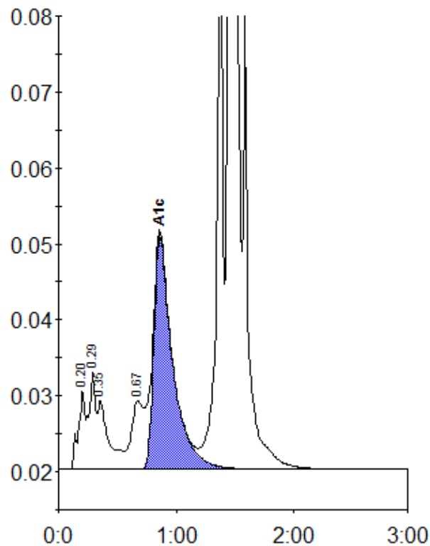
Peak table - ID: 10099787
