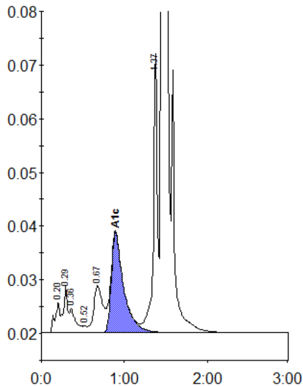
Peak table - ID: 10100086
