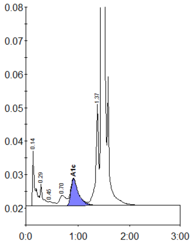
Peak table - ID: 10101063
