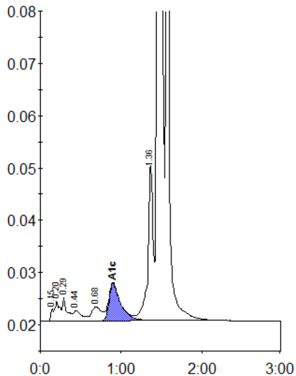
Peak table - ID: 10103240
