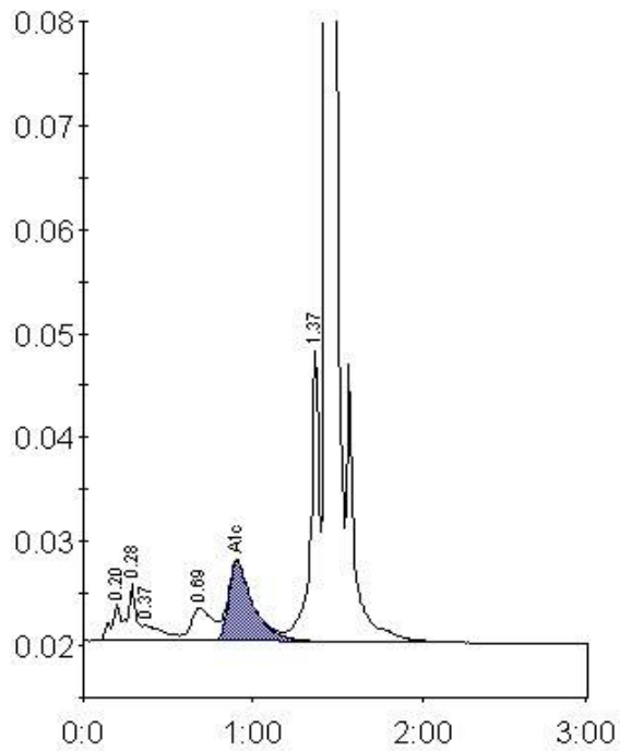
Peak table - ID: 10105399
