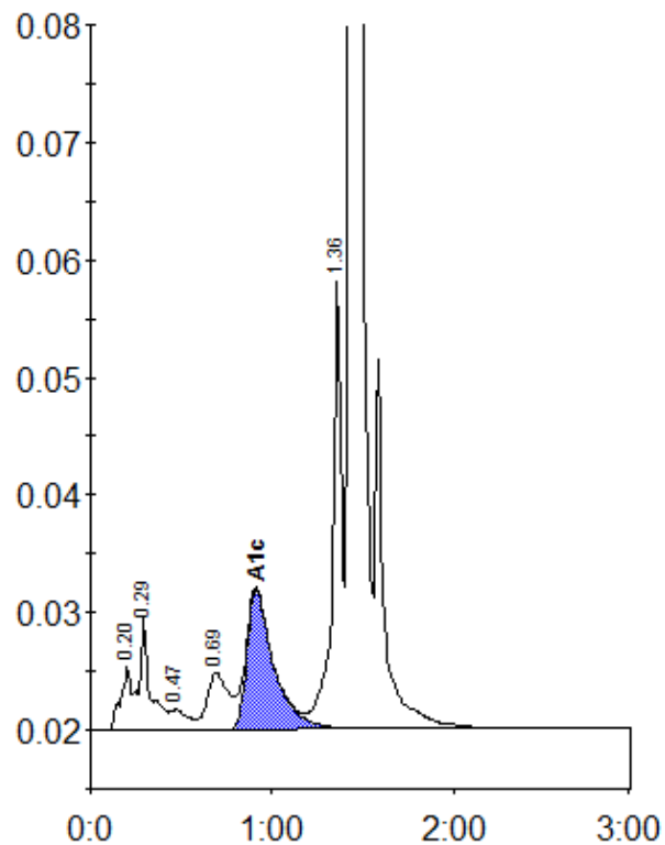
Peak table - ID: 10106165
