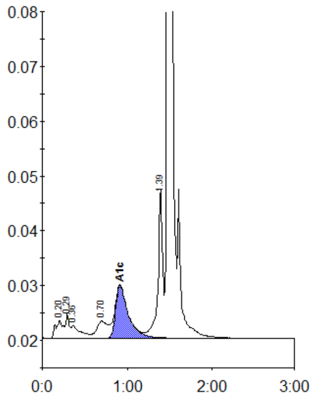
Peak table - ID: 10111656
