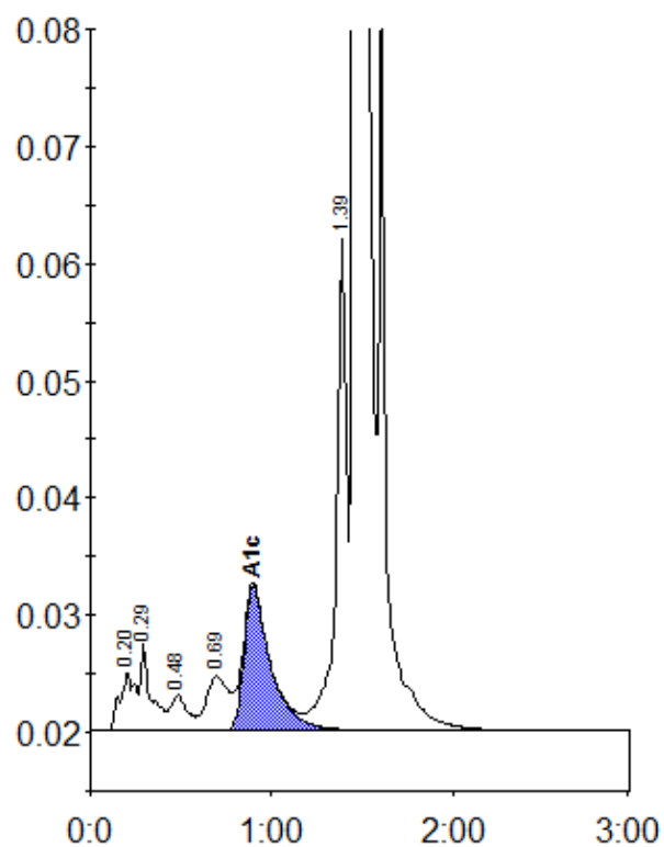
Peak table - ID: 10112100
