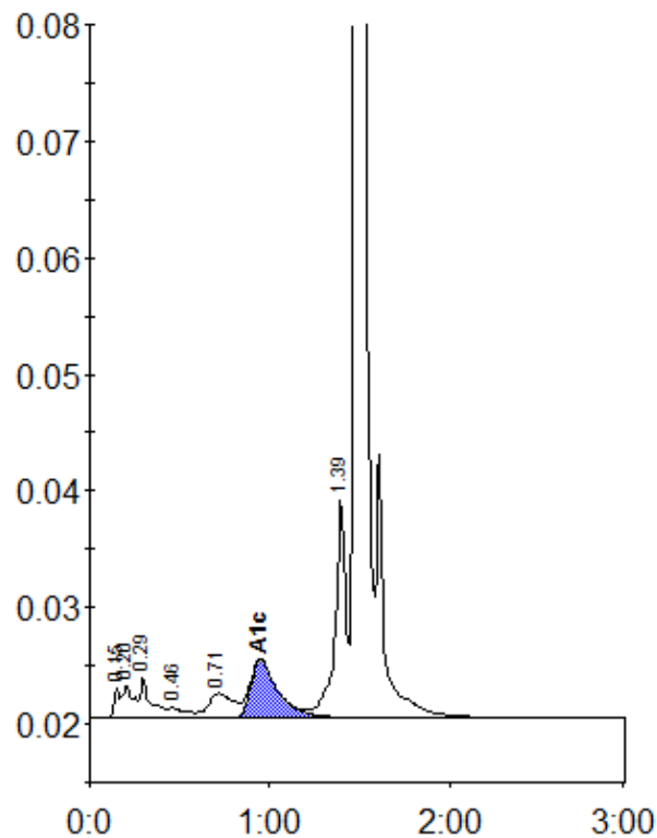
Peak table - ID: 10113183
