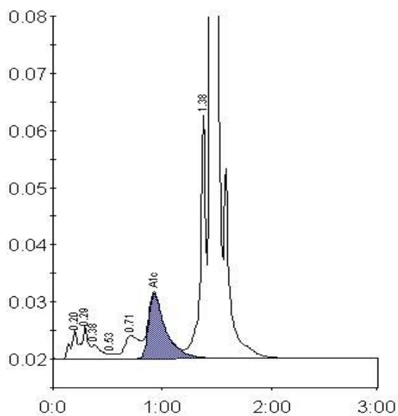
Peak table - ID: 10118375
