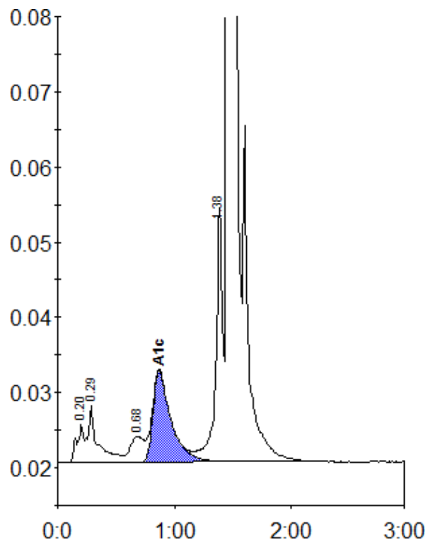
Peak table - ID: 10119862
